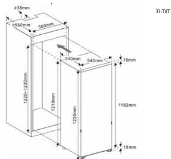
BIL1224ES scheme
