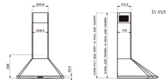
AD1046X 60cm scheme
