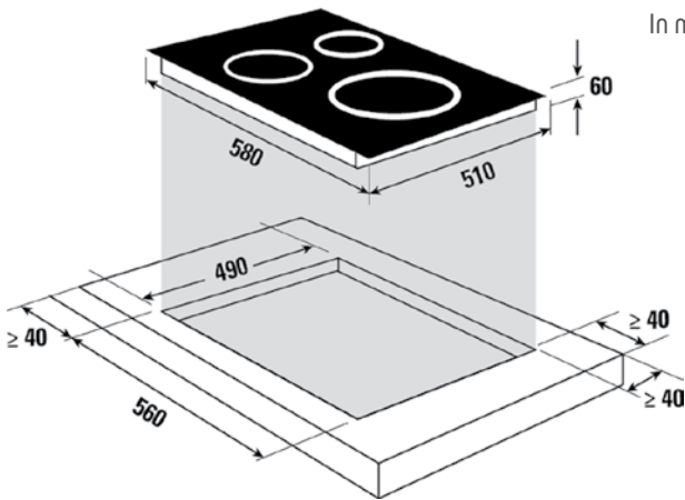
60cm Induction Hobs scheme
