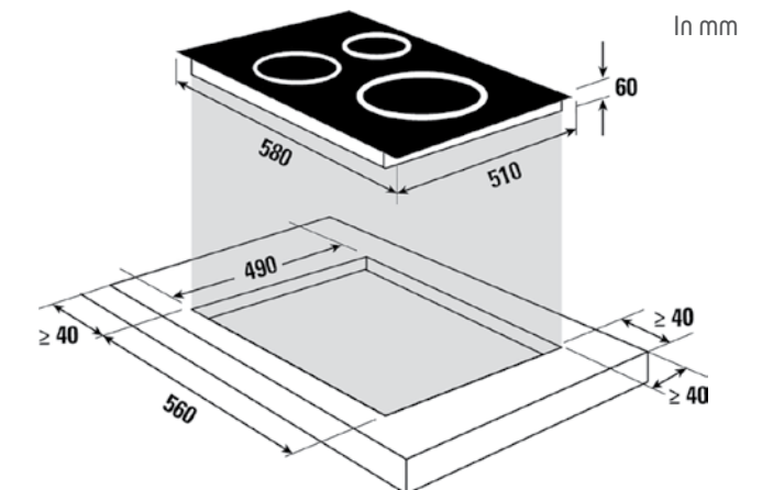
60cm Induction Hobs scheme
