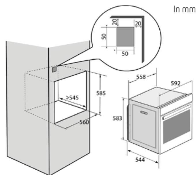
60cm Hydrolysis Ovens scheme
