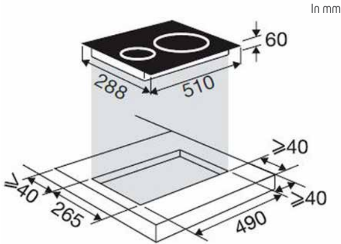
BPI1621UB & BPI6210B 30cm scheme
