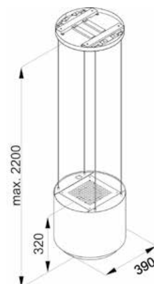
BHI2353G 38cm scheme
