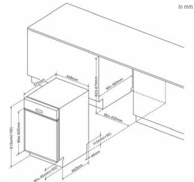
45cm Built-in Dishwasher scheme
