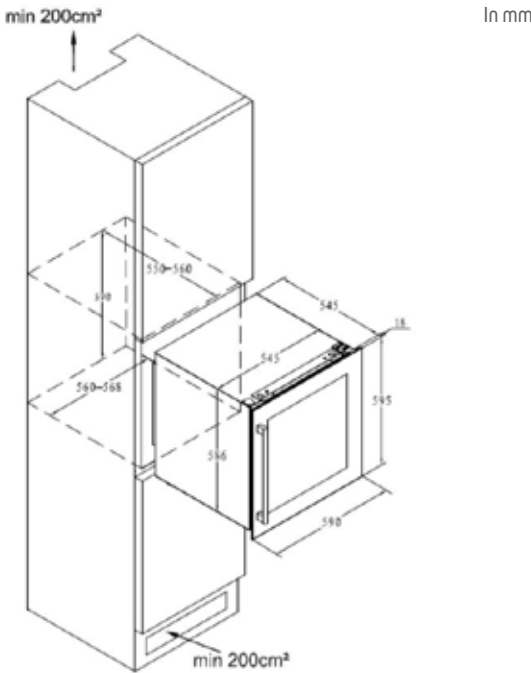
BIW36FB scheme
