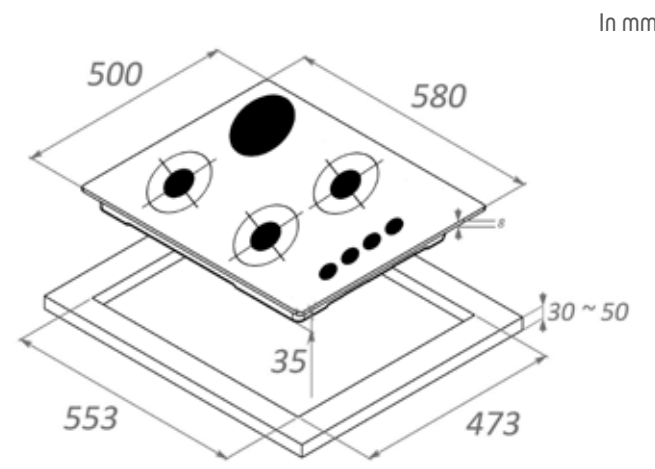
BPG3400BM Glass Hob scheme
