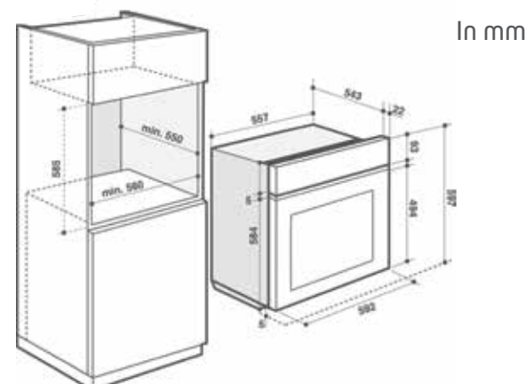
BOH1222BB/X Oven scheme
