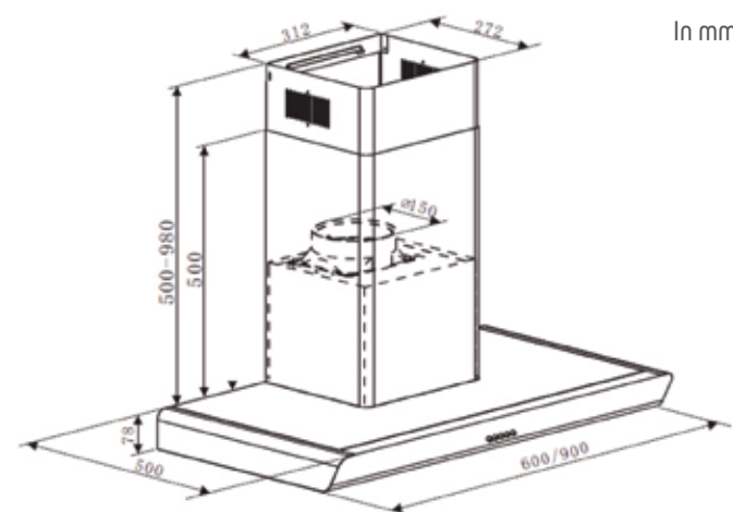
BHB6902X 90cm scheme
