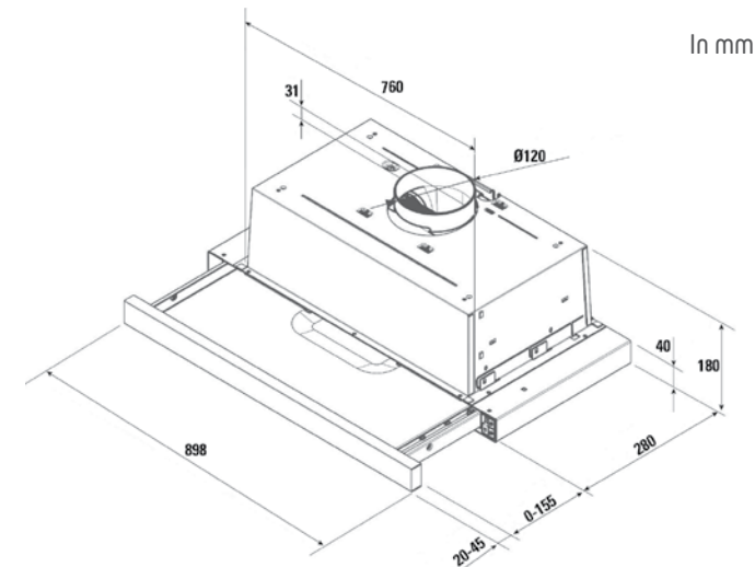
AT1349X 90cm scheme
