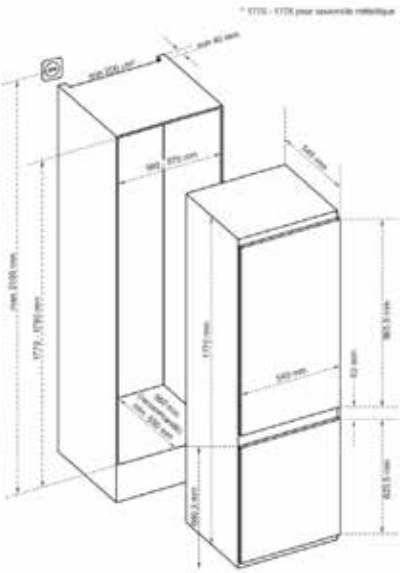
BIC7756EN scheme
