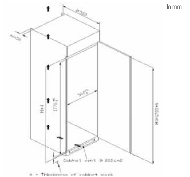
BIF7855EN scheme
