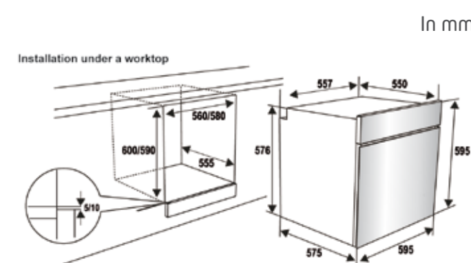
BOE1000X Oven scheme
