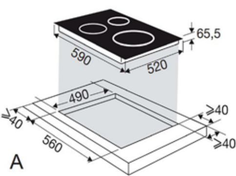
BPI6362B Hob scheme
