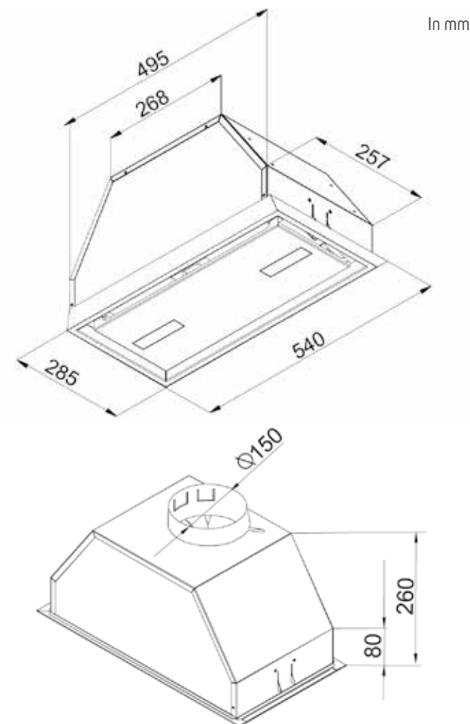
BHG2552B 54cm scheme
