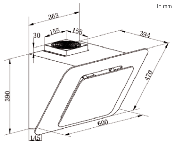
BHV1674IB 60cm scheme
