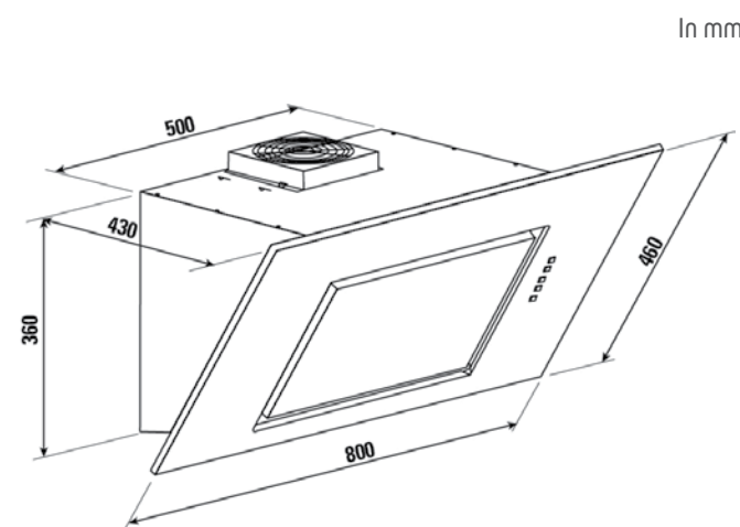
BHV6801X 80cm scheme
