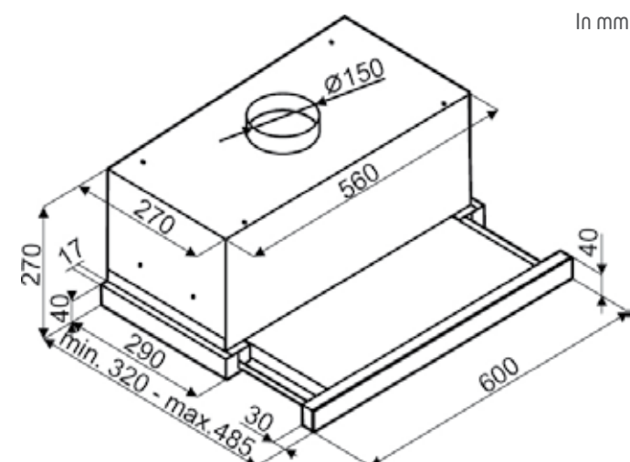
BHT2611B 60cm scheme
