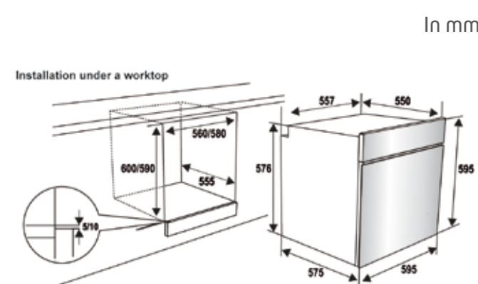
BOE1120X Oven scheme
