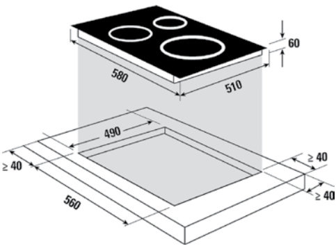
BPI2638UB Hob scheme
