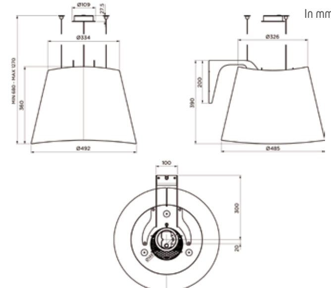
BHI1043X 49cm scheme
