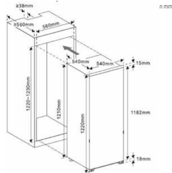
BIL1220ES scheme
