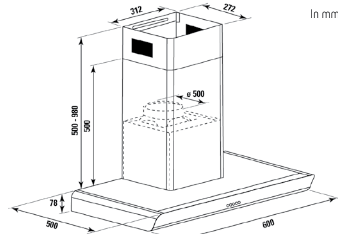
BHB6602X 60cm scheme
