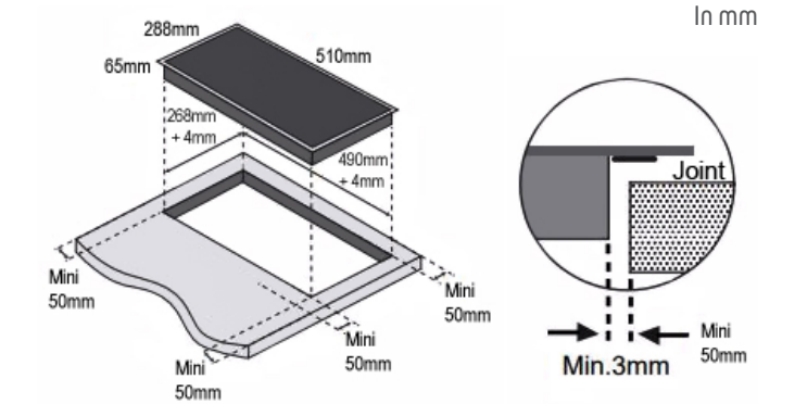
BPV6210B & BPV6222B 30cm scheme
