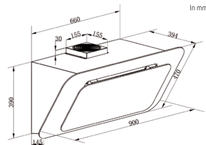
BHV1974IB 90cm scheme
