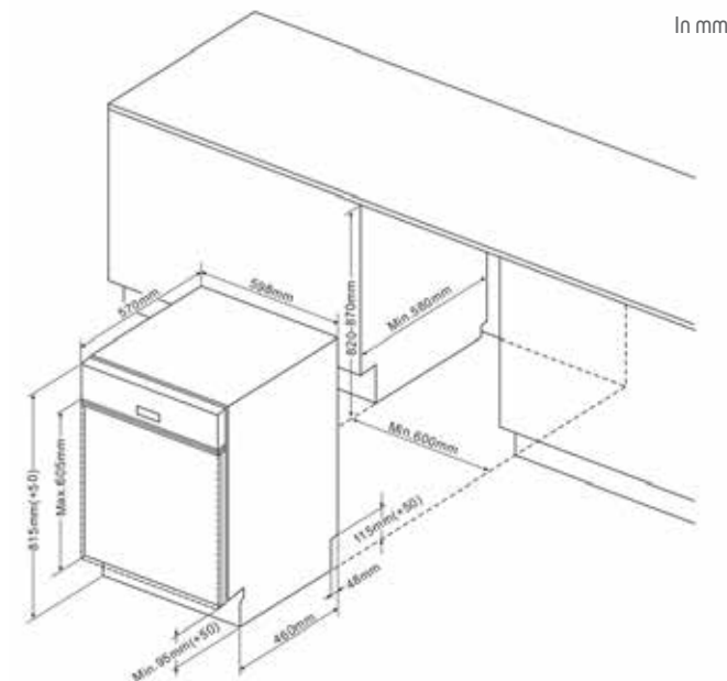
60cm Built-in Dishwashers scheme
