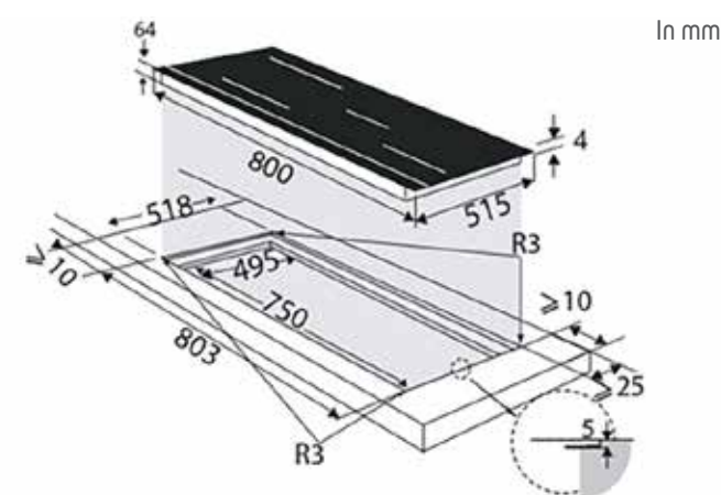
BPI384HUB 80cm scheme
