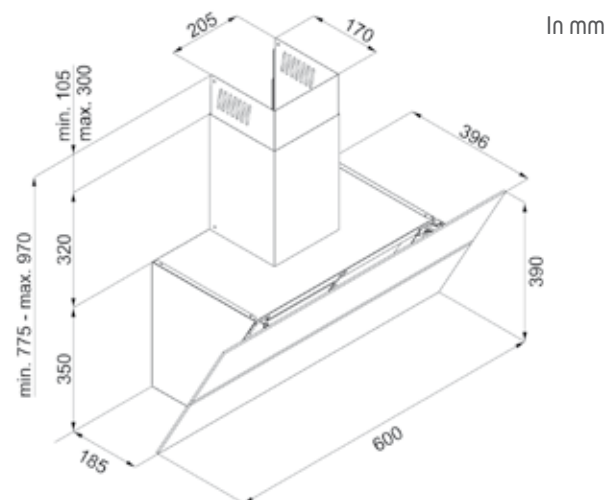
BHV2673XB 60cm scheme
