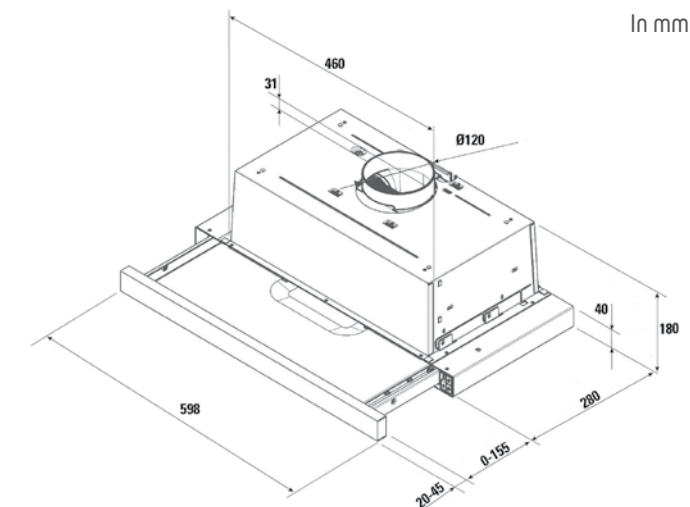
AT1346X 60cm scheme
