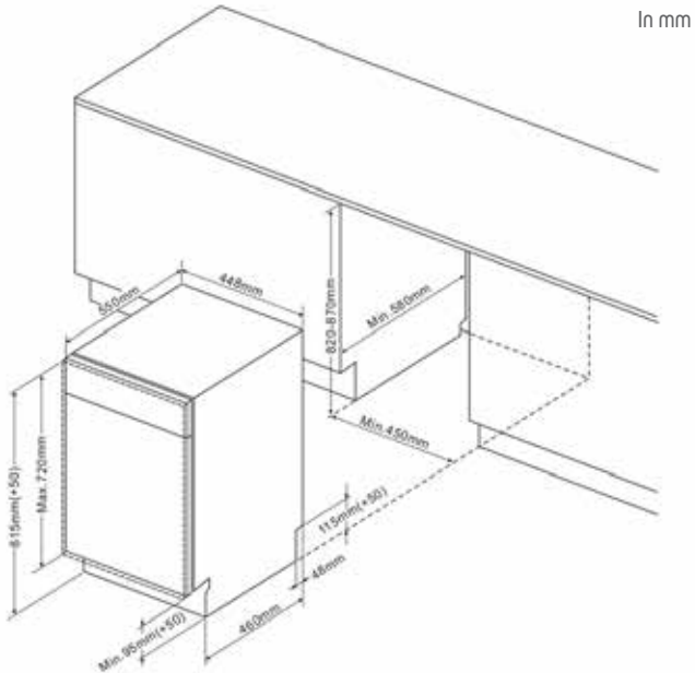
45cm Full Built-in Dishwashers scheme
