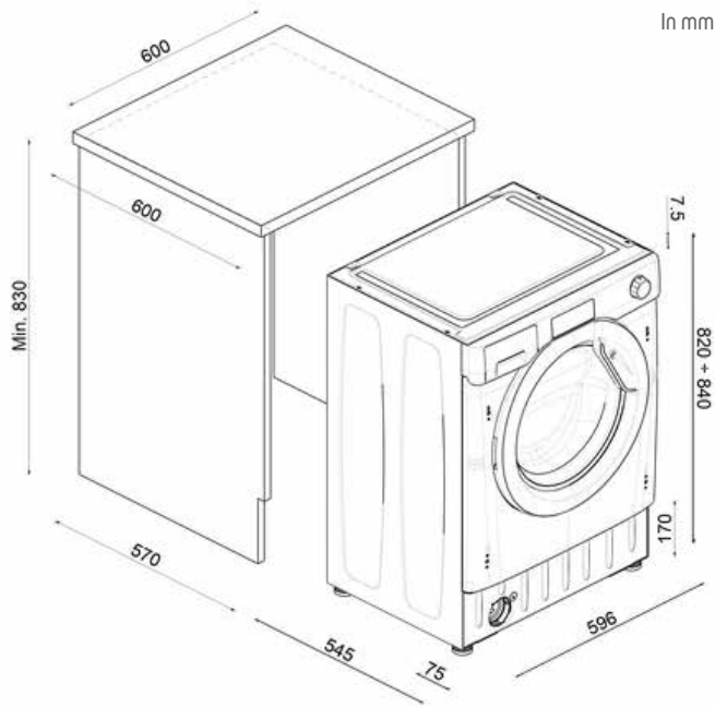
WFB484QJE scheme
