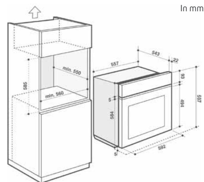
60cm Steam combination Oven scheme
