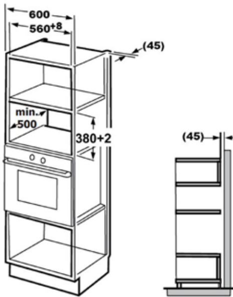
38cm 25 litres Microwaves scheme
