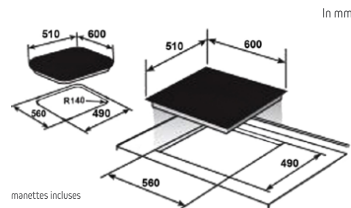
BPV2320B Hob scheme
