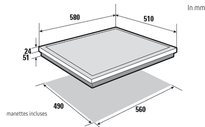
BPV6320B Hob scheme
