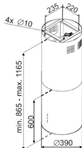
BHY2353B 38cm scheme
