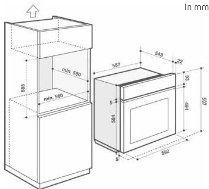
BOP7332B Oven scheme
