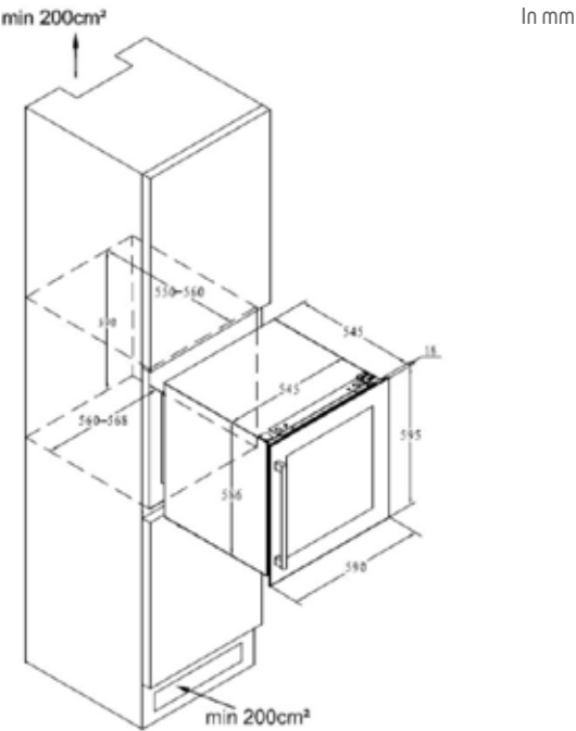
BIW28FB scheme
