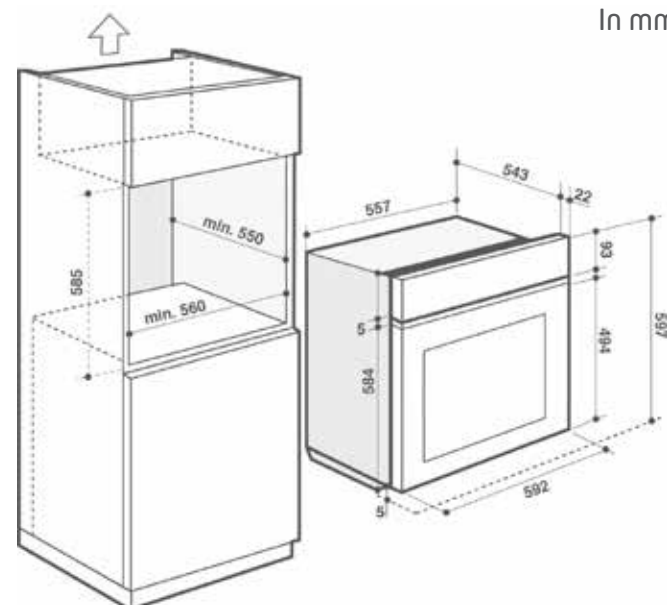
60cm Pyrolysis Ovens scheme
