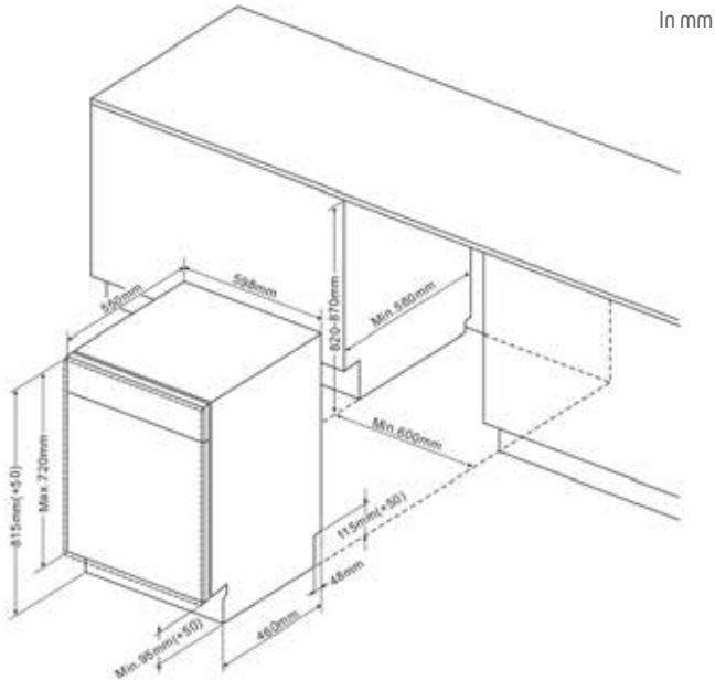
60cm Full Built-in Dishwashers scheme
