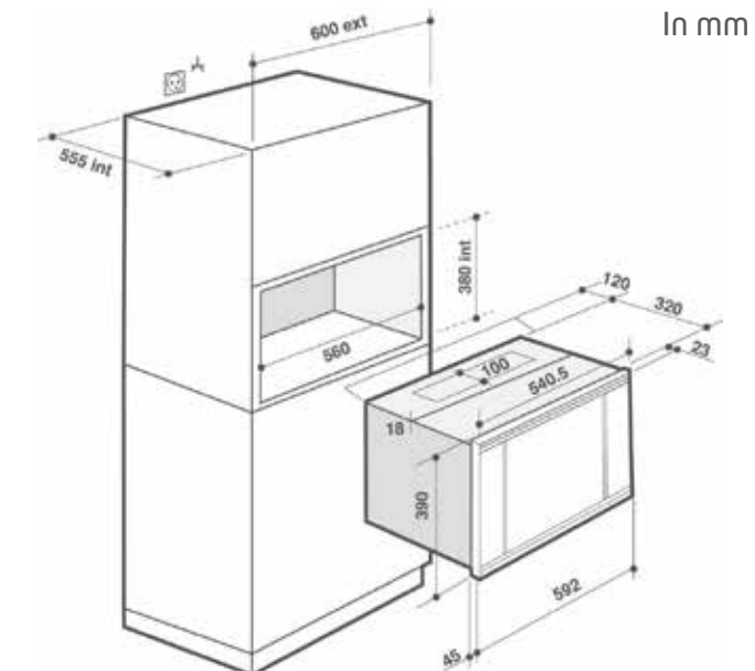
BMS7112X/B scheme
