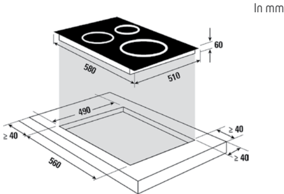
BPI6420B Hob scheme
