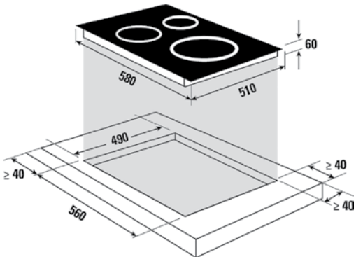
BPI2641B Hob scheme
