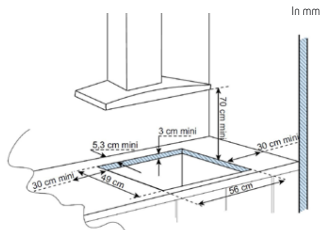
BPG6413BM Glass Hob scheme
