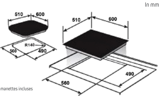
BPV1641B & BPV2421B Hobs scheme
