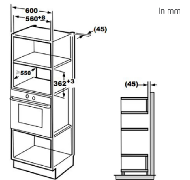
BMS6112X & BMS5112X scheme
