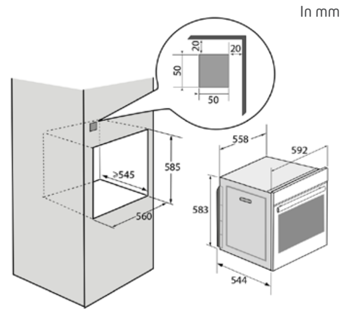
BOP2438B/BB, BOP2432X & BOP2112B Ovens scheme
