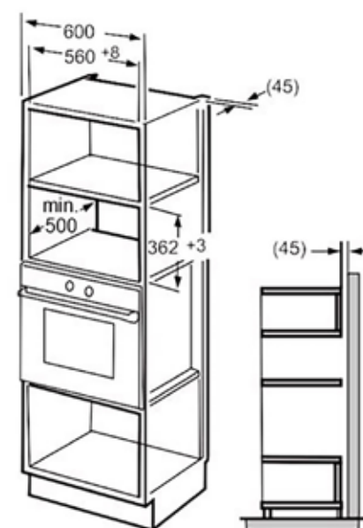
BMG2508B scheme
