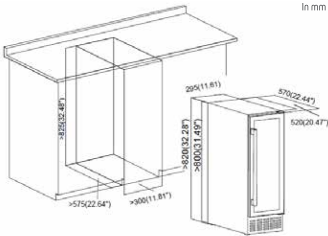
BUW20FB scheme
