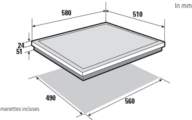
BPV6420B & BPV6410B Hobs scheme
