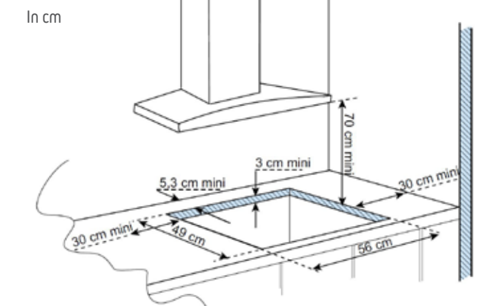
BPE6410B/X/W Hobs scheme
