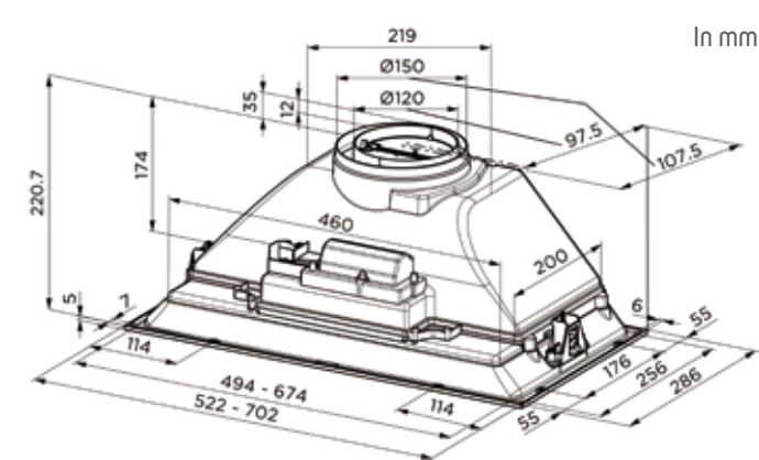
BHG1522X 52cm scheme
